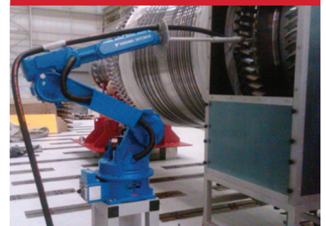
Programmable robotic peening
